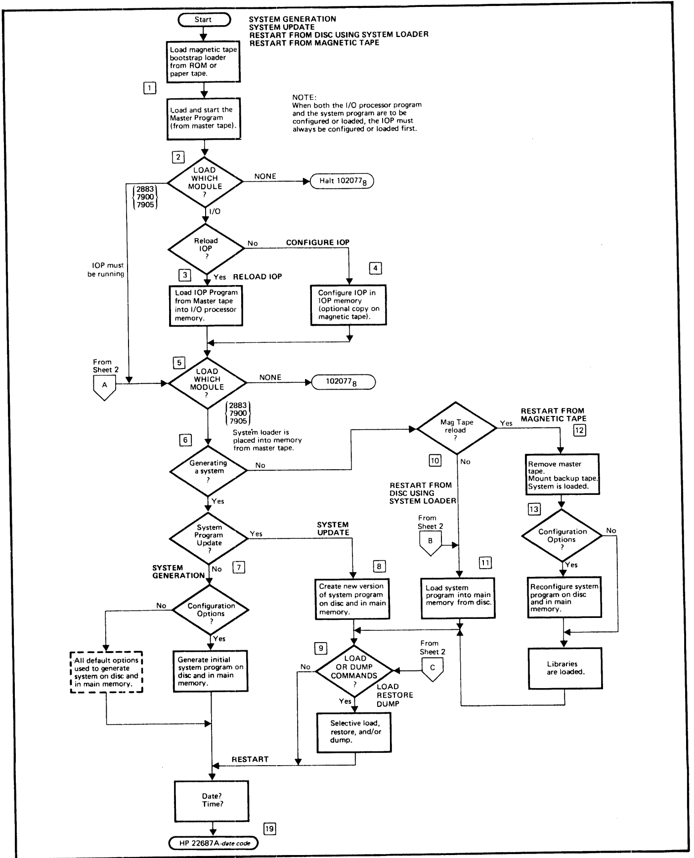
Figure 4-1. Operating Procedures Overview, Flow Diagram (Sheet 1 of 2)
