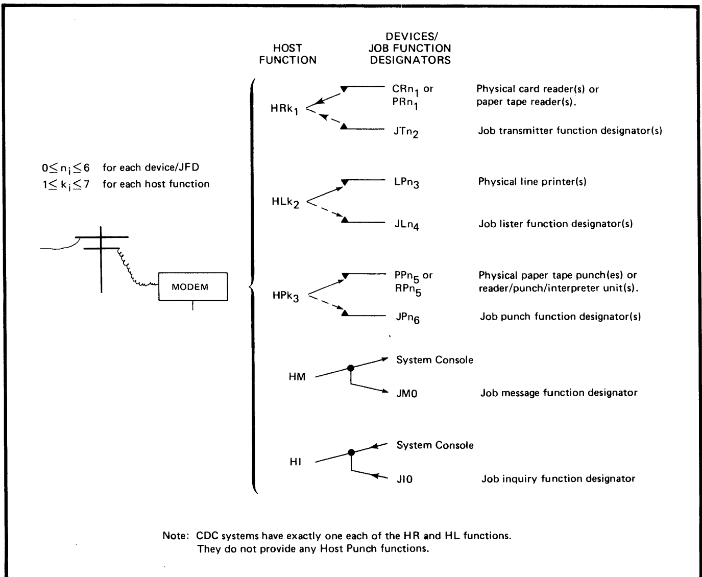
Figure 6-2. Host Function Organization
