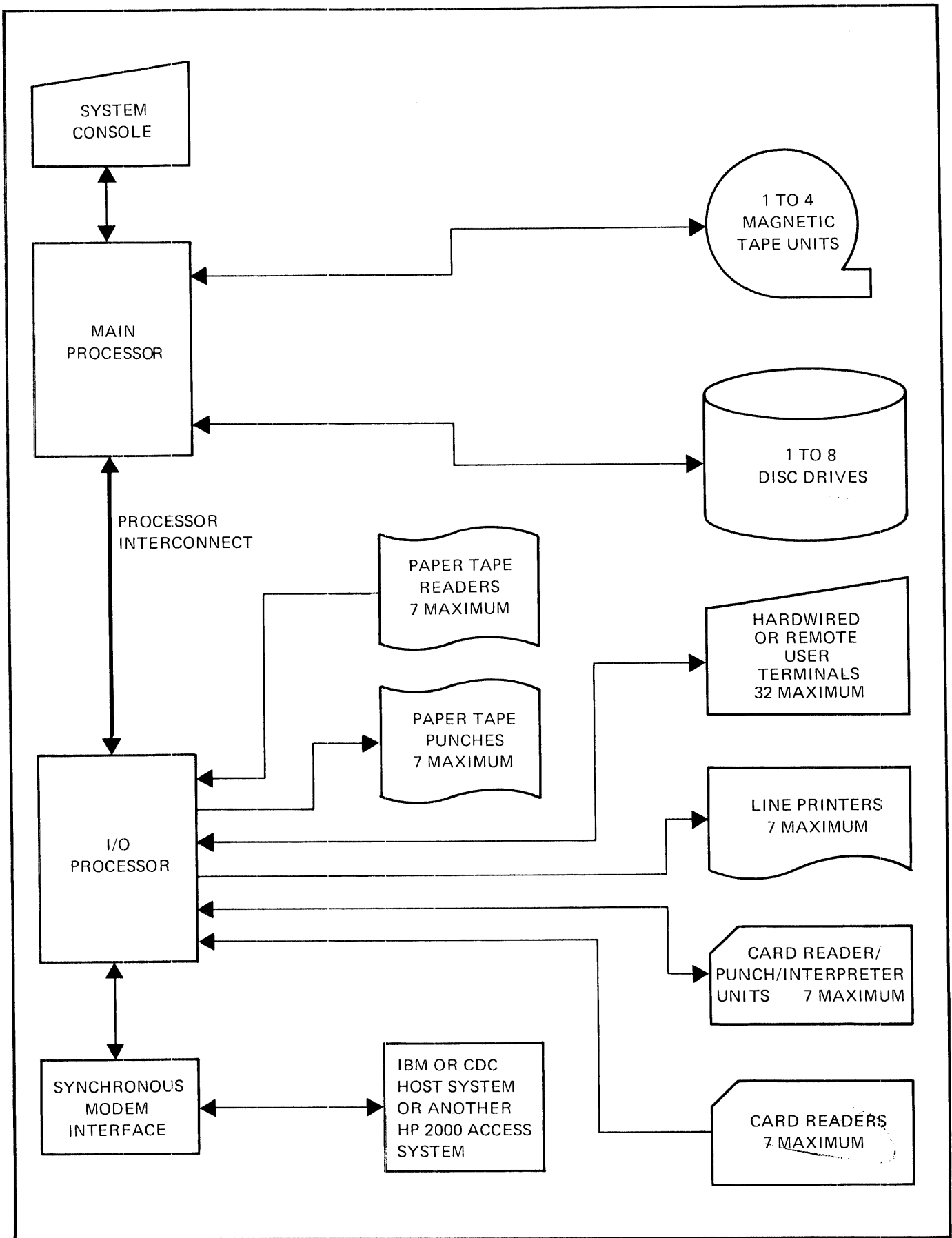
Figure 1-1. HP 2000 Access System Organization
